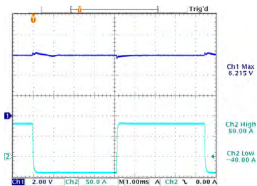
SM18-220 with Power Sink Option Current -40\text{ A} means the load delivers 40\text{ A} to the power supply (sink operation)
