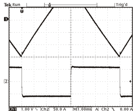
SM15-400 without Power Sink Option The output voltage is out of control when the output current is negative
