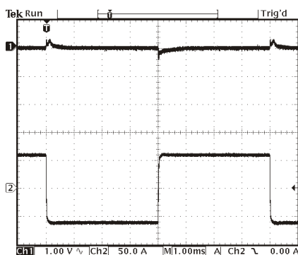
SM15-400 with Power Sink Option Current - 60 A means the load delivers 60 A to the power supply (sink operation)
