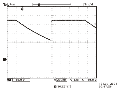
SM45-70D without Power Sink Option slow response time during voltage step down, time needed to discharge the output capacitors trace: output voltage Voltage Programming Speed at NO LOAD
