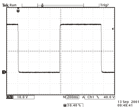
SM45-70D with Power Sink Option fast discharge of output capacitors by the power sink circuit trace: output voltage Voltage Programming Speed at NO LOAD
