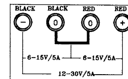
DUAL OR SERIESMODE
