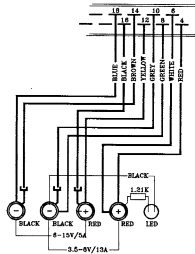
TWO ISOLATED OUTPUTS ( REMOVE RC FILTER )
