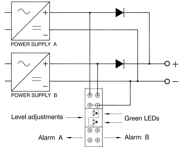
Monitoring two power supplies in redundant operation.
